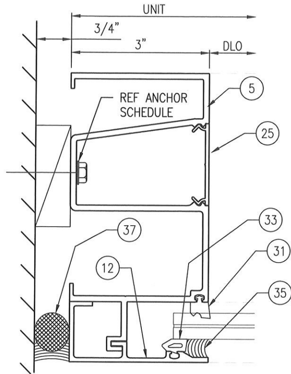
4 JAMB - CAPTURED 9/16" GLAZING Scale: 6" = 1'-0"
