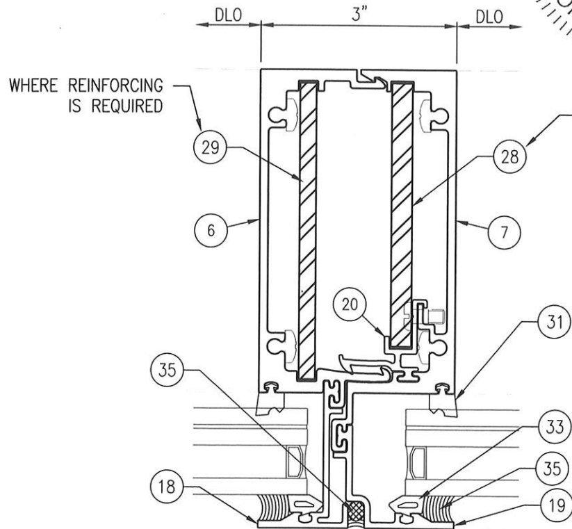
5A MULLION - CAPTURED 1-5/16" GLAZING Scale: 6" = 1'-0"
