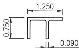
23 SUN-422 SETTING CHAIR 6063-T6
