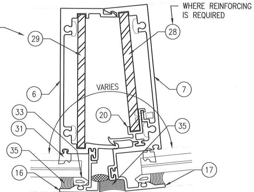
6 MULLION - CAPTURED (SPLAYED) 9/16" GLAZING Scale: 6" = 1'-0"
