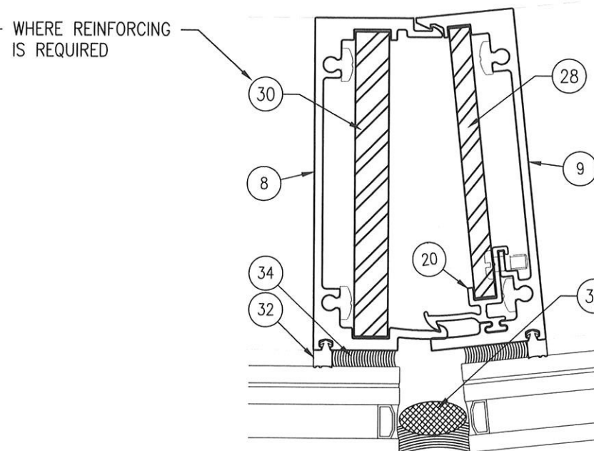
8A MULLION - BUTT GLAZED (SPLAYED) 1-5/16" GLAZING Scale: 6" = 1'-0"
