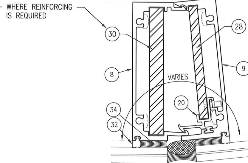
8 MULLION - BUTT GLAZED (SPLAYED) 9/16" GLAZING Scale: 6" = 1'-0"
