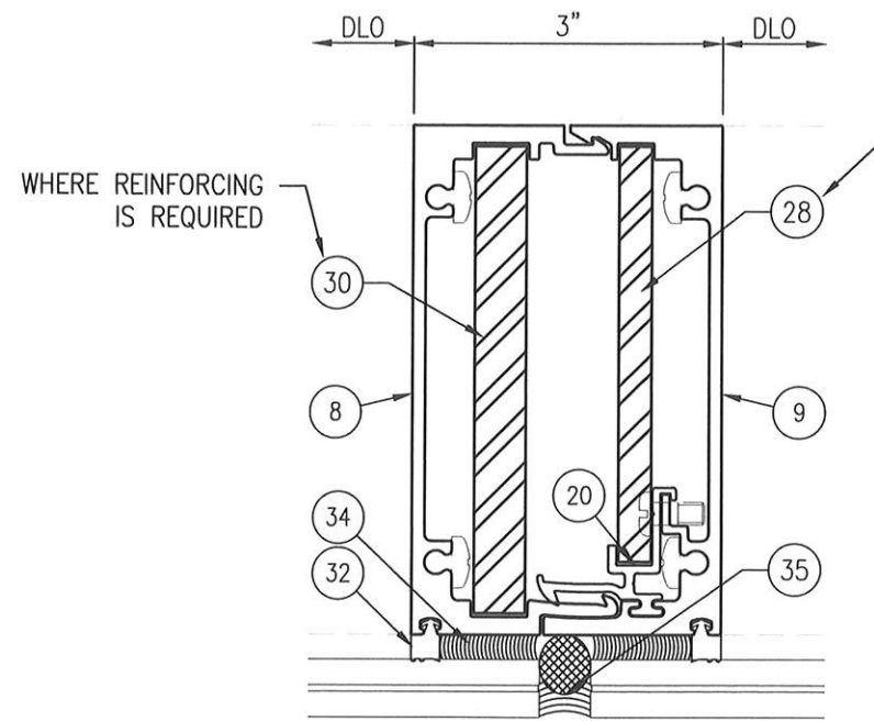
7 MULLION - BUTT GLAZED 9/16" GLAZING Scale: 6" = 1'-0"
