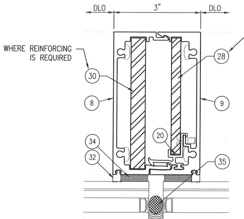
7A MULLION - BUTT GLAZED 1-5/16" GLAZING Scale: 6" = 1'-0"
