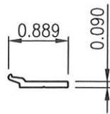
26 SUN-6132 SETTING CHAIR 6063-T6
