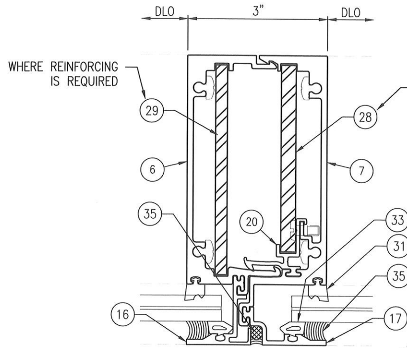
5 MULLION - CAPTURED 9/16" GLAZING Scale: 6" = 1'-0"
