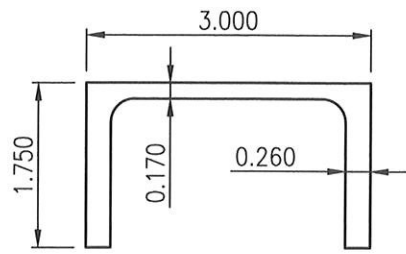
22 C3 X 1.75 X .170/.260 ANCHOR CHANNEL 6005-T5
