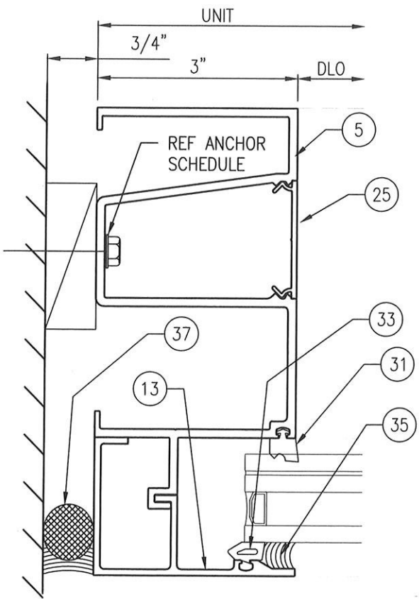
4A JAMB - CAPTURED 1-5/16" GLAZING Scale: 6" = 1'-0"
