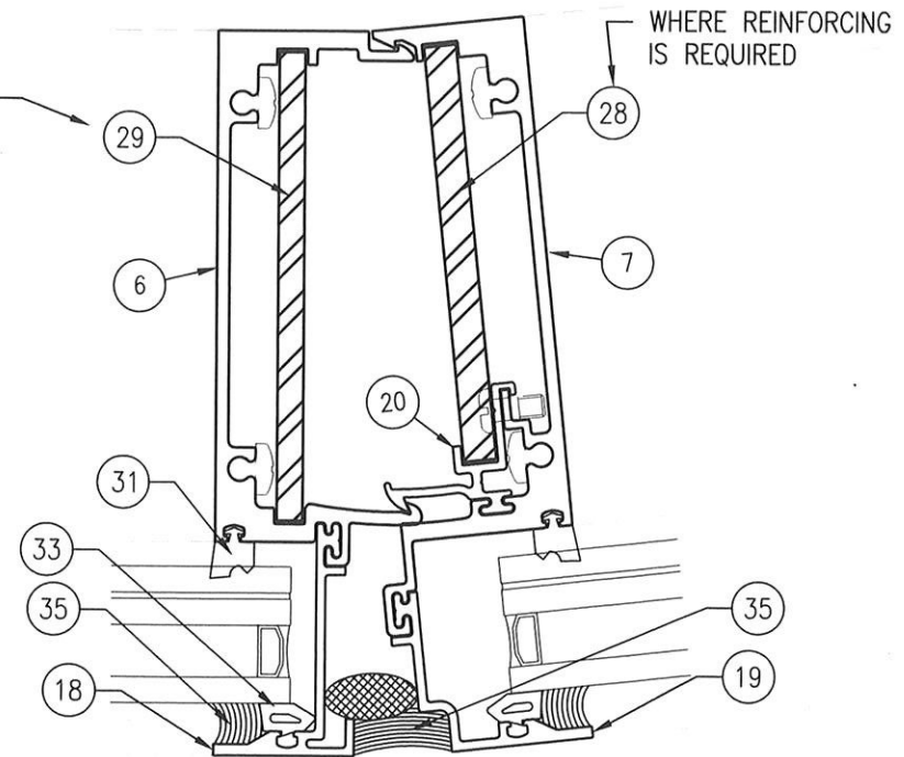
6A MULLION - CAPTURED (SPLAYED) 1-5/16" GLAZING Scale: 6" = 1'-0"
